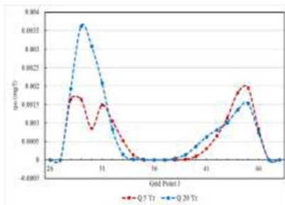
FIGURE 14 Suspended sediment Concentration section A-A
