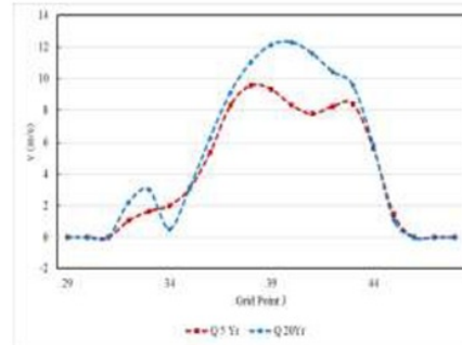
FIGURE 10 Velocity of sections B-B
