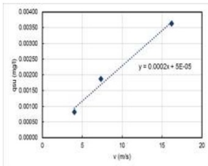
FIGURE 20 Relations between floating suspended sediment concentration and velocity at Q-20 Yr
