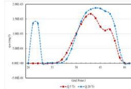
FIGURE 16 Suspended sediment Concentration section C-C
