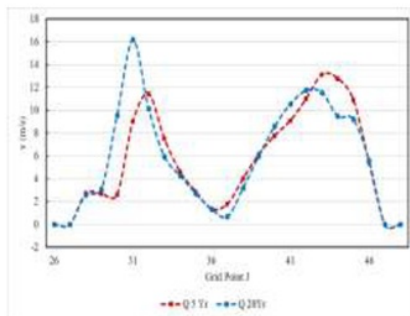
FIGURE 9 Velocity of sections A-A
