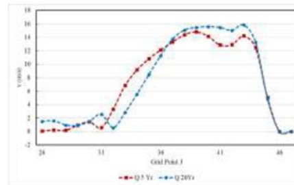
FIGURE 11 Velocity of sections C-C
