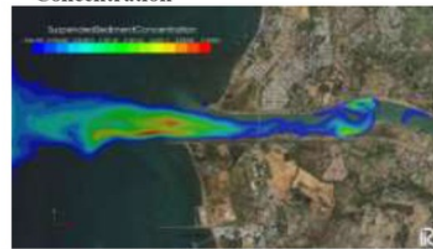
FIGURE 12 Suspended sediment Concentration t=3720 on Q-5 Yr
