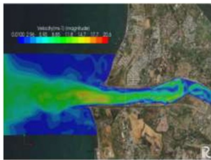
FIGURE 8 Velocity t=3720 Q 20-Yr
