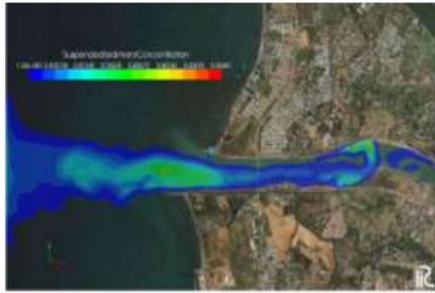
FIGURE 13 Suspended sediment Concentration t=3720 on Q-20Yr
