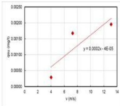
FIGURE 19 Relations between floating suspended sediment concentration and velocity at Q-5 Yr
