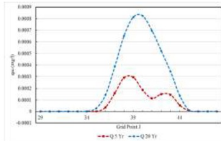
FIGURE 15 Suspended sediment Concentration section B-B
