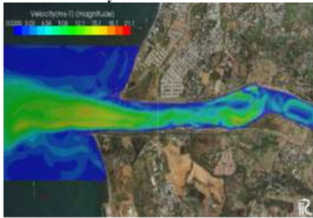
FIGURE 7 Velocity t = 3720 Q 5-Yr
